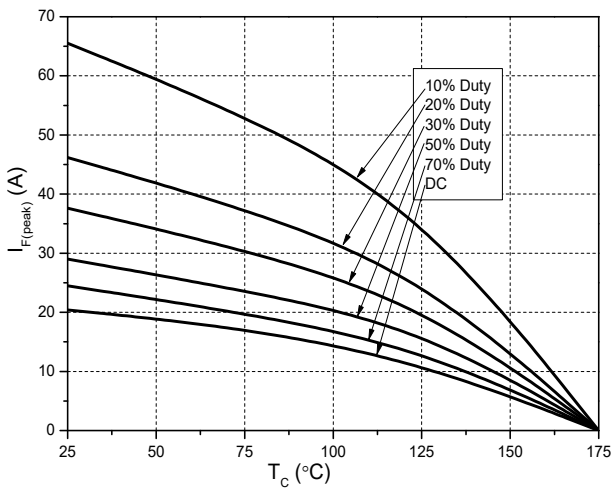
Figure 7. Current Derating
